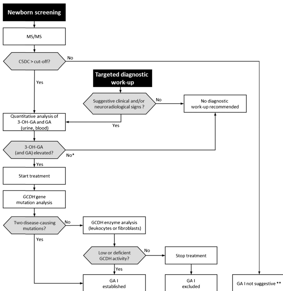
Fig. 1 Diagnostic algorithm for glutaric aciduria type I (GA-I). Newborn screening is performed using tandem mass spectroscopy (MS/MS) analyzing glutarylcarbitine (C5DC) concentration in dried blood spots (DBS). Diagnostic workup includes quantitative analysis of GA and 3-hydroxyglutaric acid (3-OH-GA) in urine and/or blood, molecular genetic analysis of GCDH gene, and glutaryl-CoA dehydrogenase (GCDH) enzyme analysis. Targeted diagnostic workup due to suggestive clinical, biochemical, and/or neuroradiological signs starts with quantitative analysis of GA and 3-OH-GA in urine and/or blood and is performed in analogy to the described diagnostic workup procedure. *Low-excretors may show (intermittently) normal concentrations of 3-OH-GA (and GA) in urine or blood. If highly suspicious signs and symptoms for GA-I are
